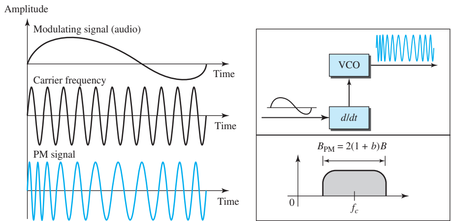
Figure 5.20 Phase modulation
